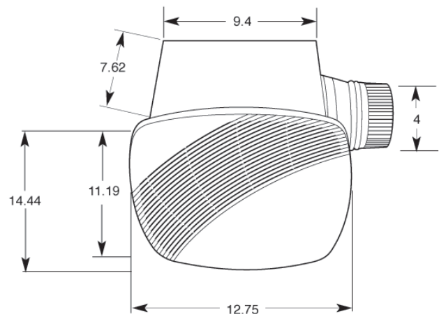
NuVent Product Performance Model NXSH110FL
