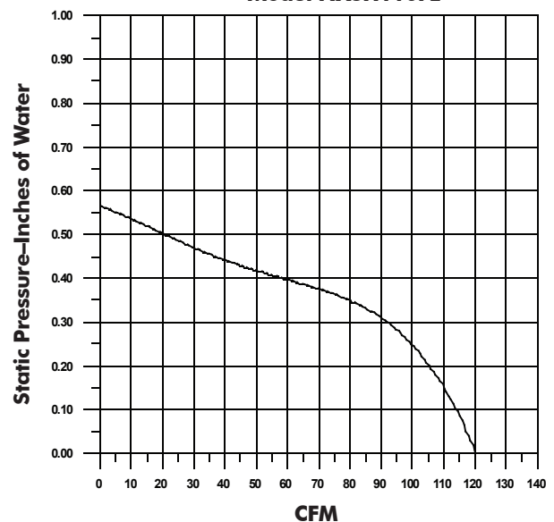
NuVent Product Performance Model NXSH110FL
